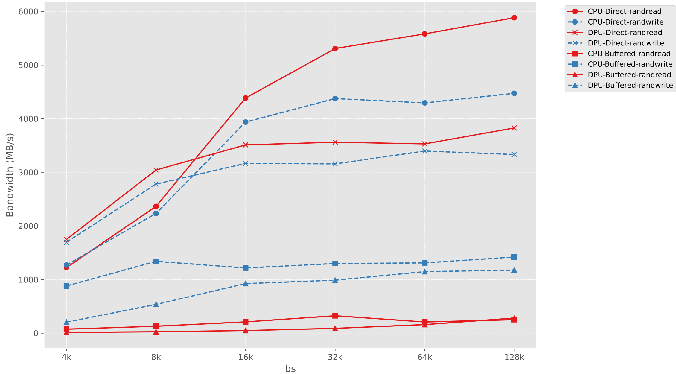
Bandwidth vs bs (CPU vs DPU, Direct vs Buffered)
